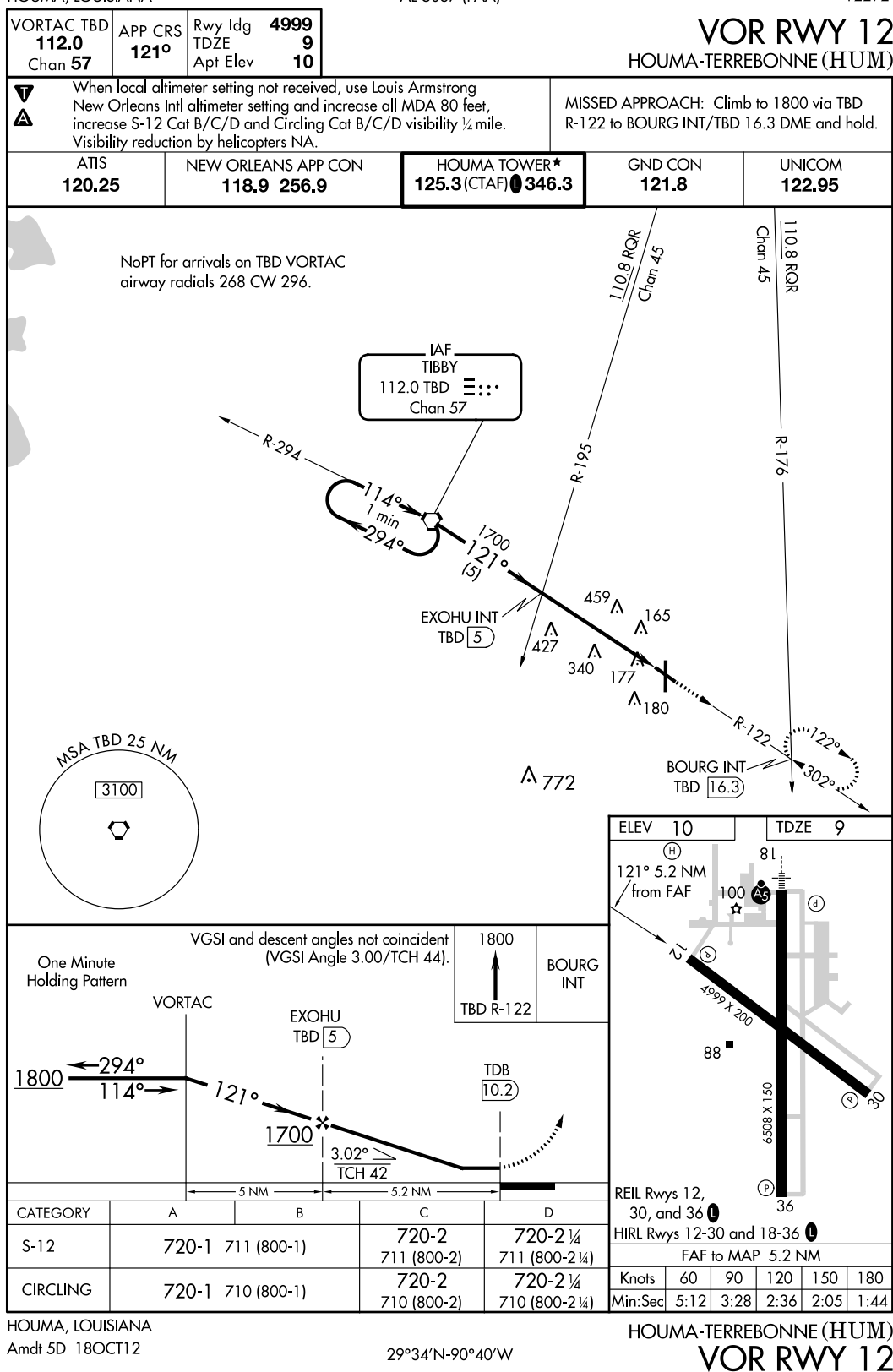
FIGURE 200.—VOR RWY 12 (HUM).
