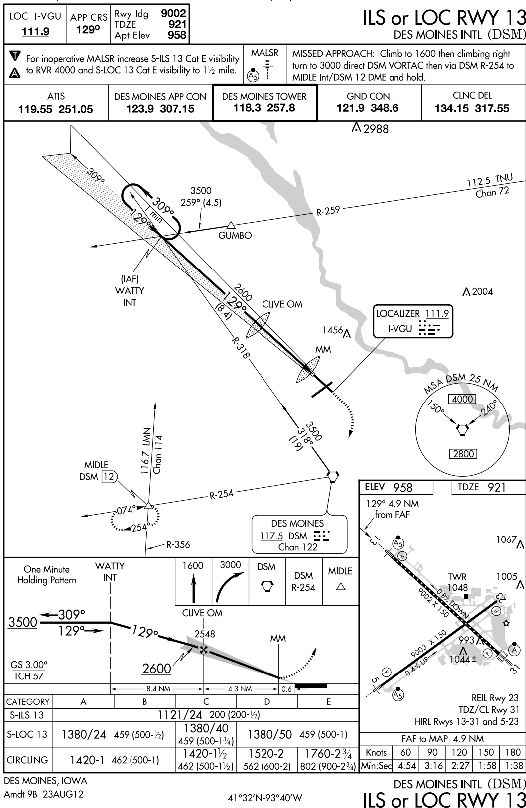
FIGURE 217.—ILS or LOC RWY 13 (DSM).
