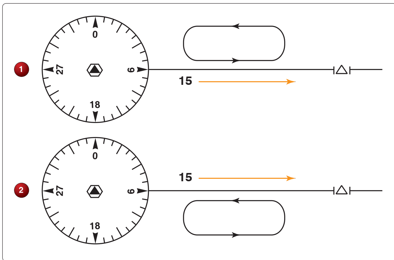
FIGURE 112.—Holding Entry Procedure.
