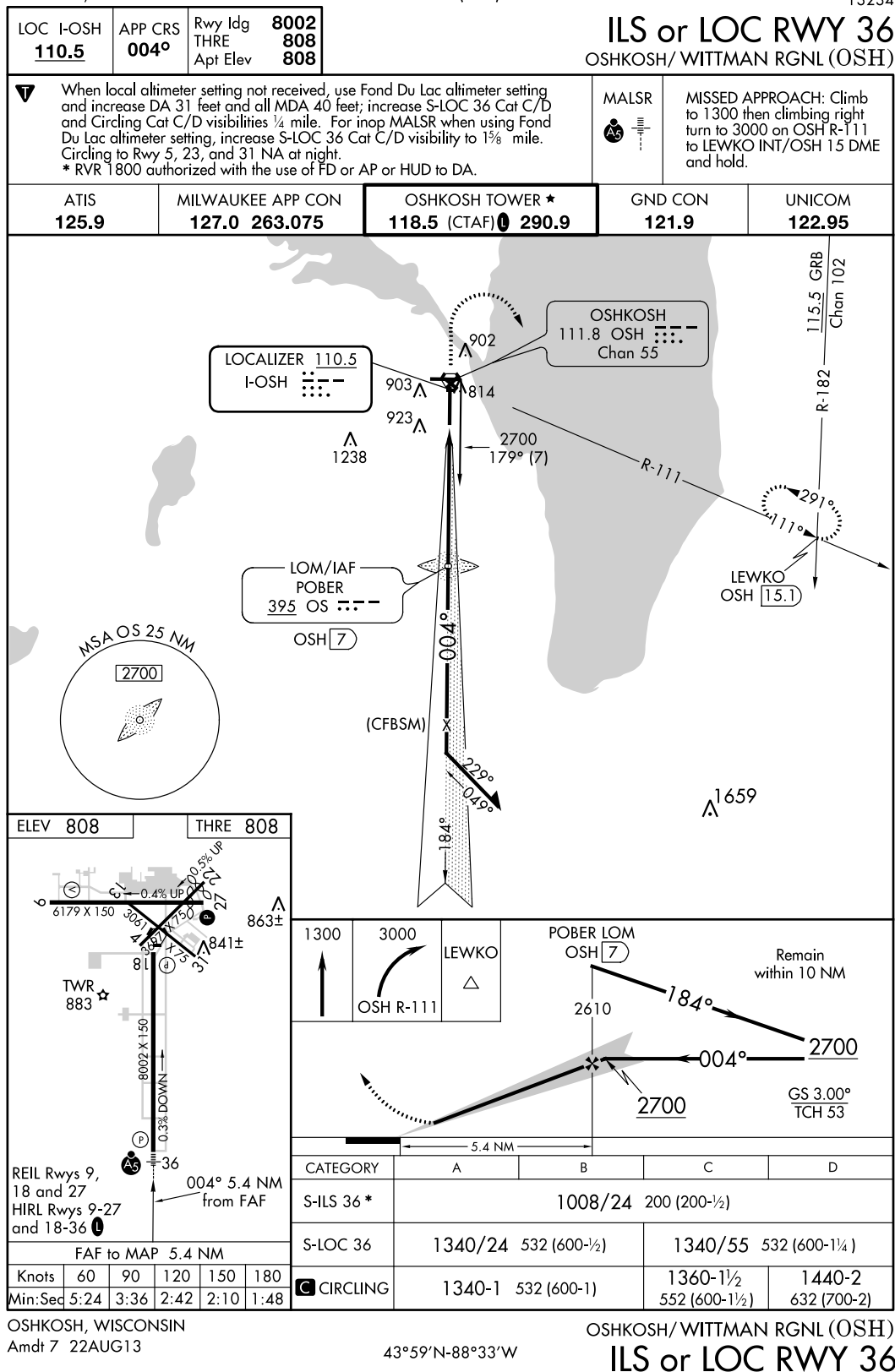
FIGURE 252.—ILS or LOC RWY 36 (OSH).
