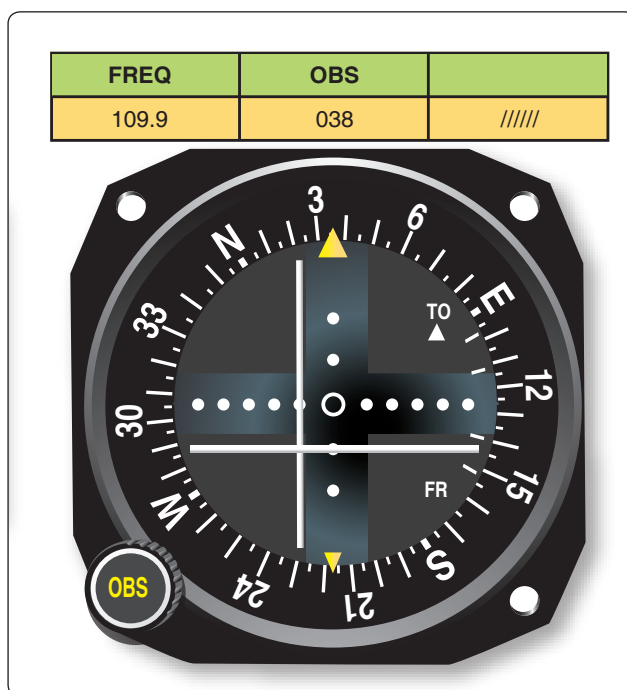
FIGURE 61.—CDI Indicator.
