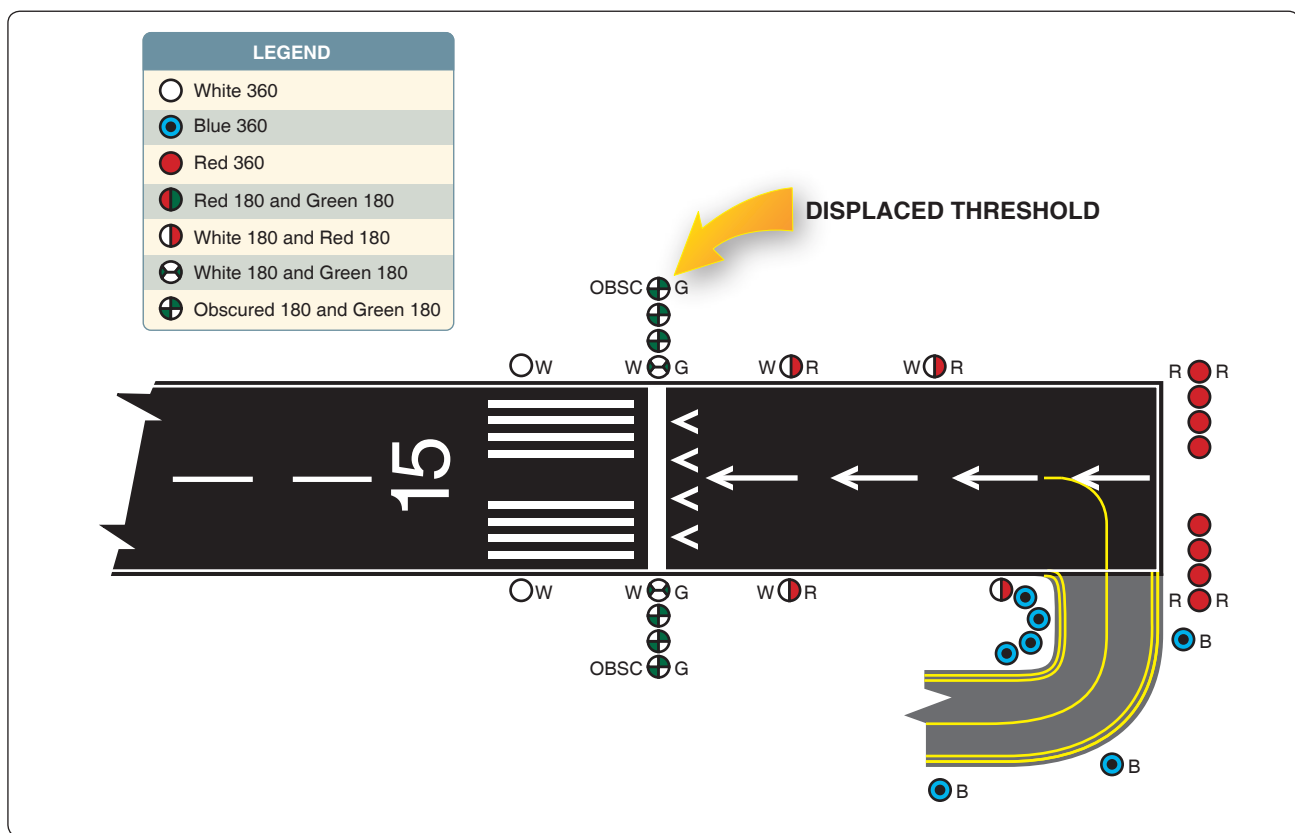
FIGURE 138.—Runway Legend.
