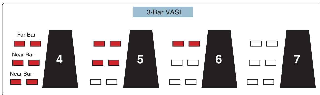
FIGURE 135.—3-BAR VASI.
