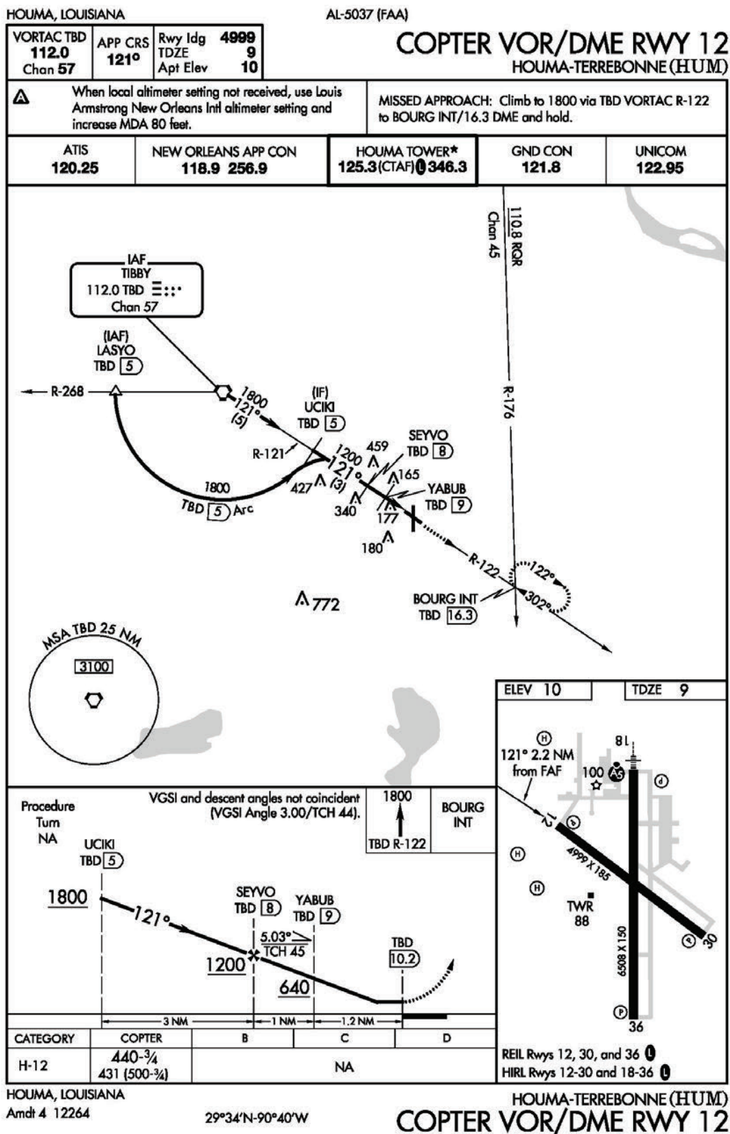
FIGURE 199.—COPTER VOR/DME RWY 12 (HUM).
