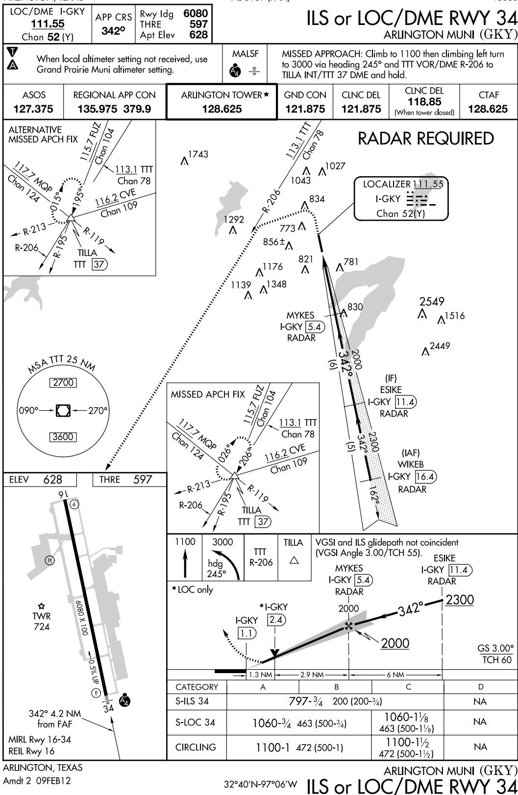
FIGURE 180.—ILS or LOC/DME RWY 34 (GKY).
