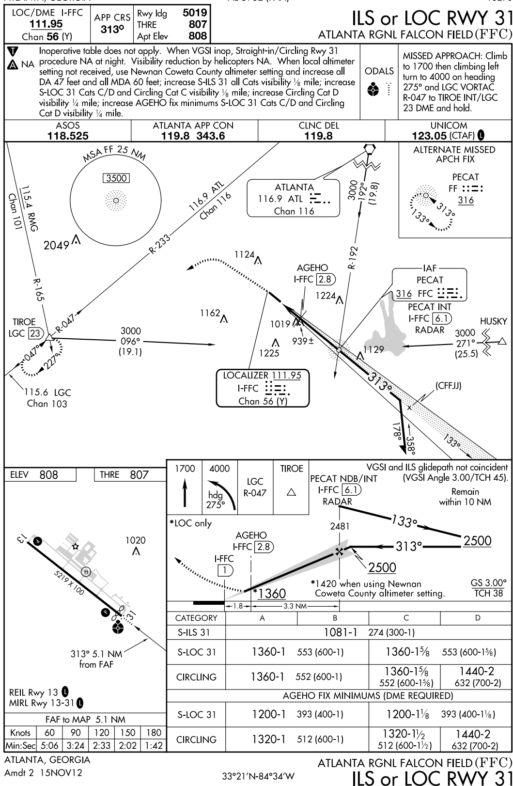
FIGURE 228.—ILS or LOC RWY 31 (FFC).
