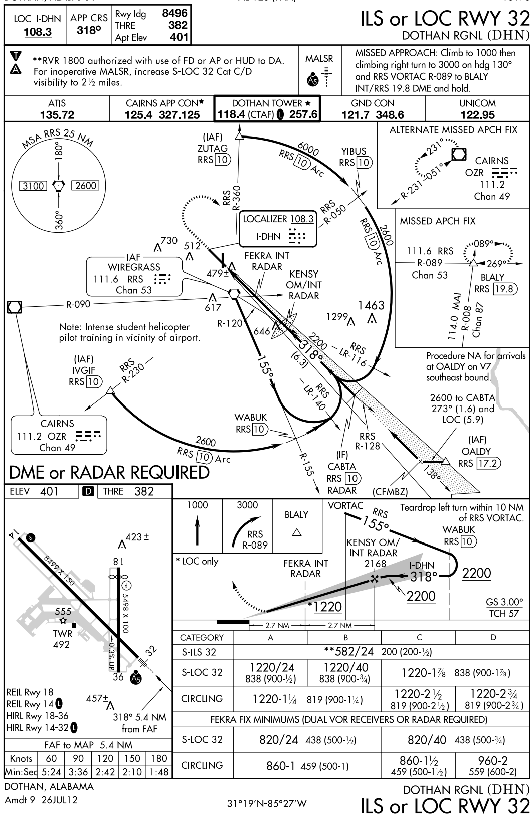
FIGURE 236.—ILS or RWY 32 (DHN).
