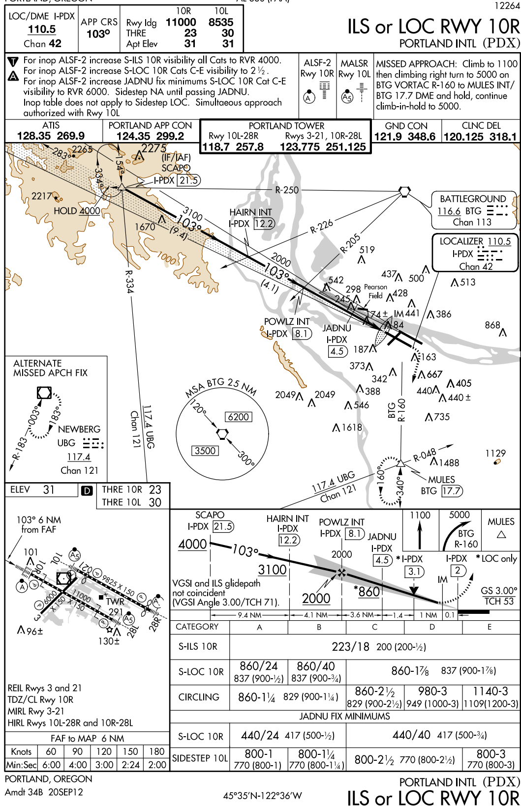
FIGURE 186.—ILS or LOC RWY 10R (PDX).
