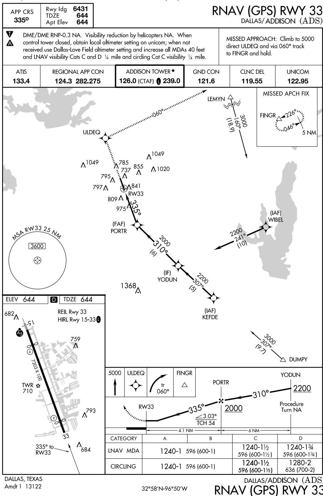
FIGURE 171.—RNAV (GPS) RWY 33 (ADS).
