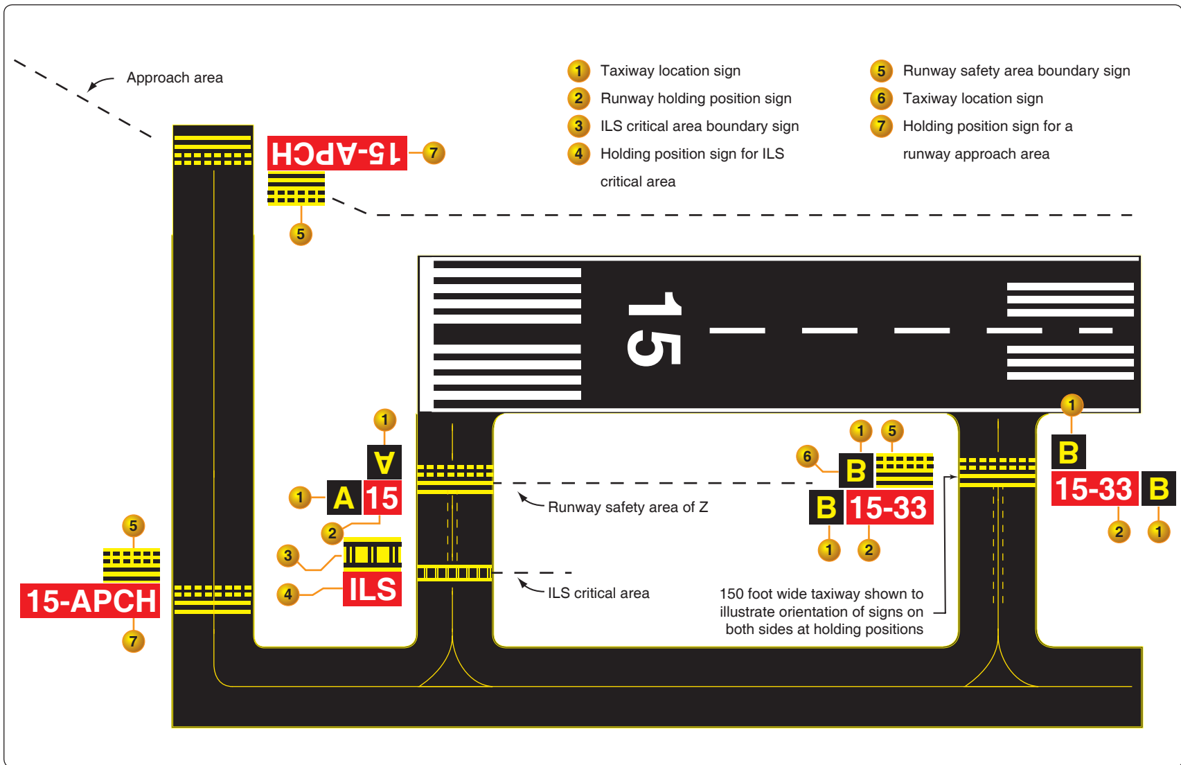
FIGURE 94.—Application Examples for Holding Positions.
